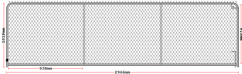
Plain Top Single Leaf Left Hinge Gate 3000mm Opening Size
