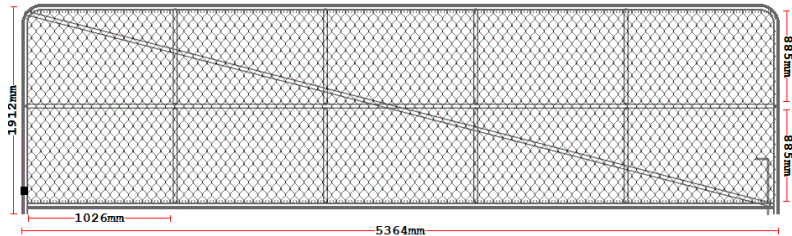
Plain Top Single Leaf Left Hinge Gate 5400mm Opening Size
