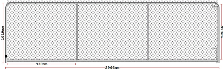
Plain Top Single Leaf Left Hinge Gate 3000mm Opening Size
